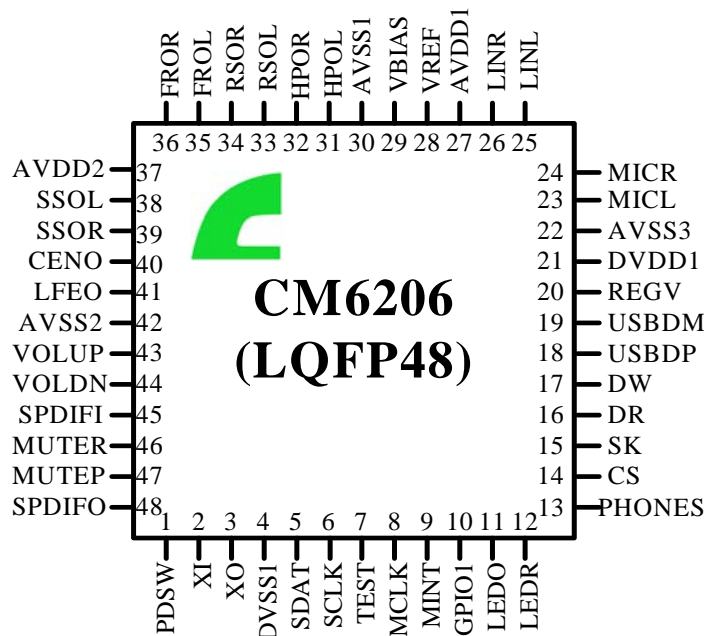
Figure 1. CM6206 LQFP 48 Pin Assignments (Top View)
